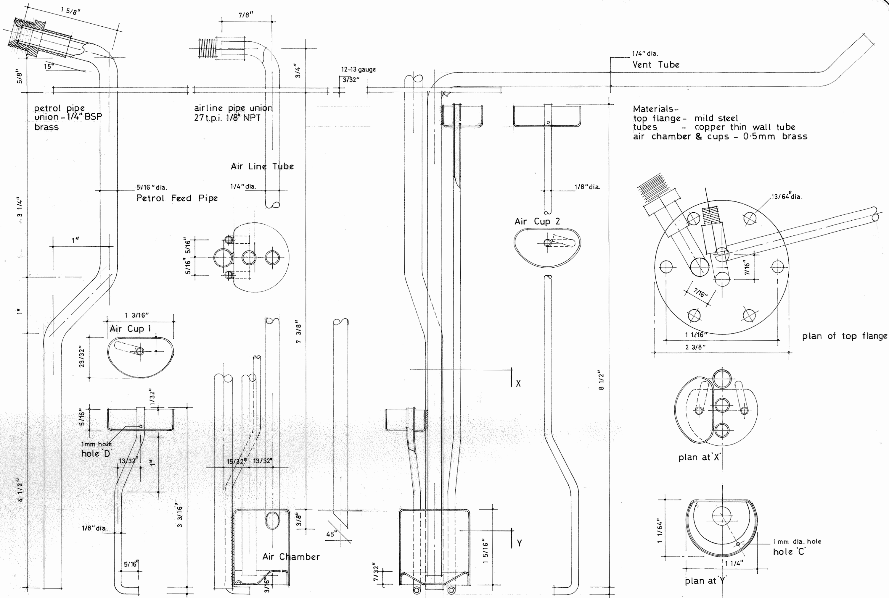
Hobson Petrol Telegage Tank Unit as fitted to Riley cars
